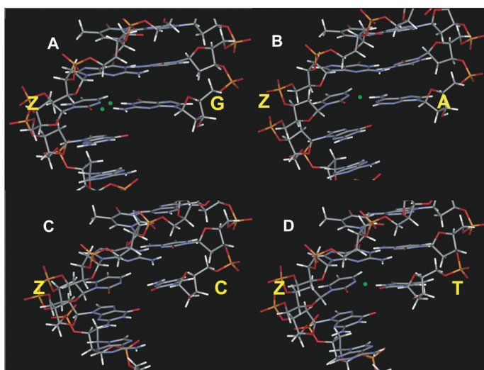
FIGURE 4 Energy-minimized primer-template DNA structures following dNTP incorporation opposite zebularine. (A) dGTP, (B) dATP, (C) dCTP, and (D) dTTP.
