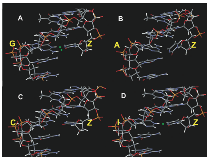
FIGURE 3 Energy-minimized primer-template DNA structures following dZTP incorporation opposite (A) guanine, (B) adenine, (C) cytosine, and (D) hypoxanthine (inosine).
